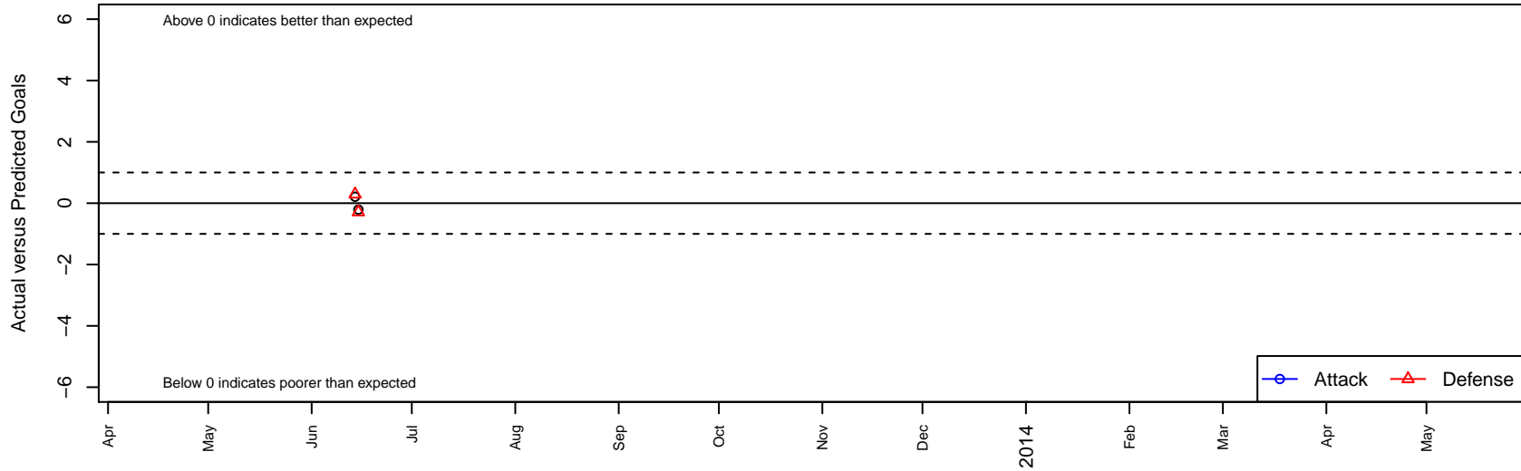
Evolution B00 Dots are actual minus expected GF (blue circles) and GA (red triangles). Blue line is smoothed change in attack strength. Red is smoothed change in defense strength.
